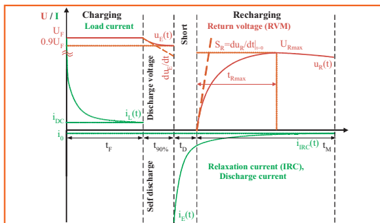
Fig. 4: Dielectric response in time base
