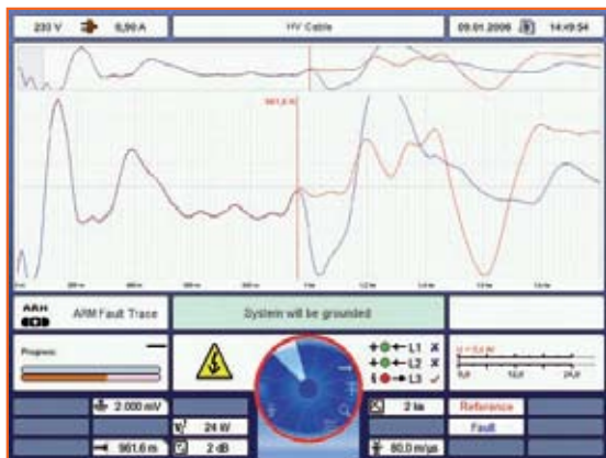
ARM*- and ARM* Plus Reflectograms
