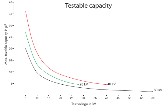
Fig. 1 Test capacitance against the test voltage
